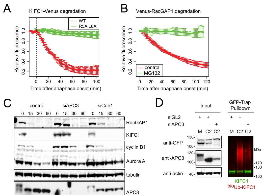
FIG. 4. KIFC1 and RacGAP1 are mitotic exit-specific APC/C substrates. A–B, Venus-tagged KIFC1 or RacGAP1 were electroporated into U2OS cells, and after 12 to 24 h mitotic cells were imaged by means of fluorescence time-lapse microscopy. Venus levels in individual mitotic cells were quantified and plotted as a function of anaphase onset. In vivo degradation curves are shown as averaged results with error bars showing standard deviations. A, KIFC1-Venus is a substrate of mitotic-exit-specific proteolysis that depends on a putative D-box (R5xxL) in the unstructured N terminus. B, Venus-RacGAP1 is a substrate of mitotic-exit-specific proteolysis, as a decrease in Venus-RacGAP1 levels did not occur in cells treated at anaphase onset with 5 \mu M MG132. See also supplemental Fig. S4 . C, depletion of APC3 stabilizes endogenous KIFC1 and RacGAP1 in mitotic exit. U2OS cells were transfected with siRNA against control (luciferase, GL2), APC3, or Cdh1 sequences, synchronized to prometaphase as described in Fig. 1D and released using CDKI/II inhibitor. Cells were harvested at the indicated time points, and whole cell lysate was examined via immunoblot with antibodies against known and putative APC/C substrates. APC3 immunoblot indicated progress of mitotic exit with reversal of marked mitotic phosphorylation shift. D, in vivo ubiquitination of KIFC1-Venus was sensitive to the depletion of APC3. KIFC1-Venus electroporated into bio Ub cells synchronized in M and C phases as in C was subjected to GFP-Trap® pull-down as described in Ref. 57. Anti-GFP immunoblot revealed unmodified KIFC1-Venus (in green), whereas anti-biotin immunoblot revealed KIFC1-Venus-associated ubiquitin conjugates (in red).
