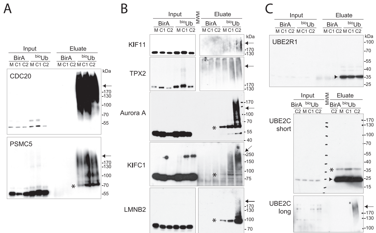
FIG. 3. Immunoblot validation of specific ubiquitin conjugates identified via mass spectrometry. A–C, loading in pulldown lanes = 1000× loading in input lanes, except for LMNB2 (700×), UBE2R1 (700×), and UBE2C (550×). Ubiquitinated material in pulldowns appears either as up-shifted monoubiquitinated bands (*) or as polyubiquitinated proteins in high-MW smears (indicated by arrows). E2 enzymes purified as ubiquitin thioester conjugates, which were reduced during elution because DTT was present, migrated at the same MW as the unmodified protein (indicated by arrowheads). A, Cdc20 and PSMC5 (Sug1) were strongly polyubiquitinated in all fractions. B, mitotic regulators KIF11, TPX2, AURKA, and KIFC1, as well as nuclear lamin LMNB2, were present as polyubiquitin conjugates specific to mitotic exit fractions. Where input and eluate are shown in separate panels, the eluate panel was taken from a longer exposure of the same blot. See supplemental Fig. S3 for full-size blots and additional validations. Mono-ubiquitination of Aurora A (*) has not previously been described. C, E2 enzymes UBE2R1 and UBE2C were strongly enriched in bio Ub pulldowns, with UBE2C additionally polyubiquitinated late in mitotic exit (long exposure).
